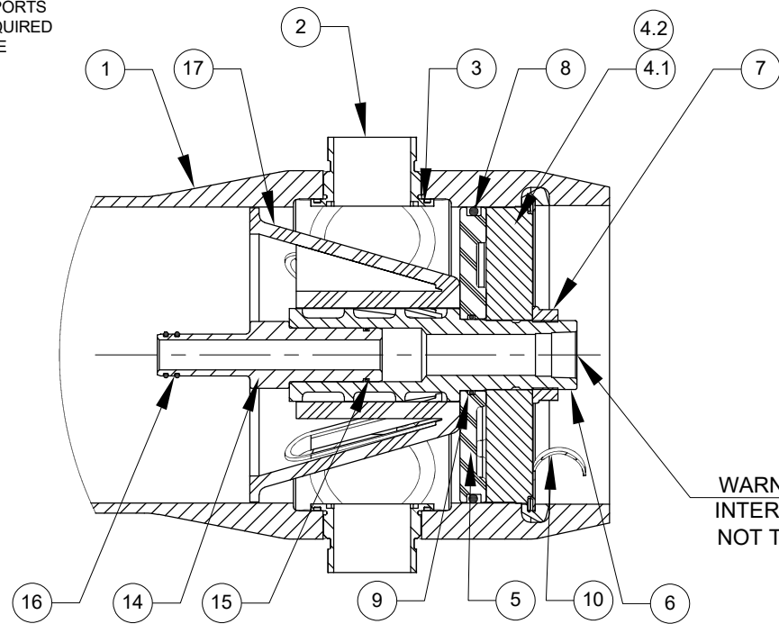
SECTION THROUGH END CLOSURE
